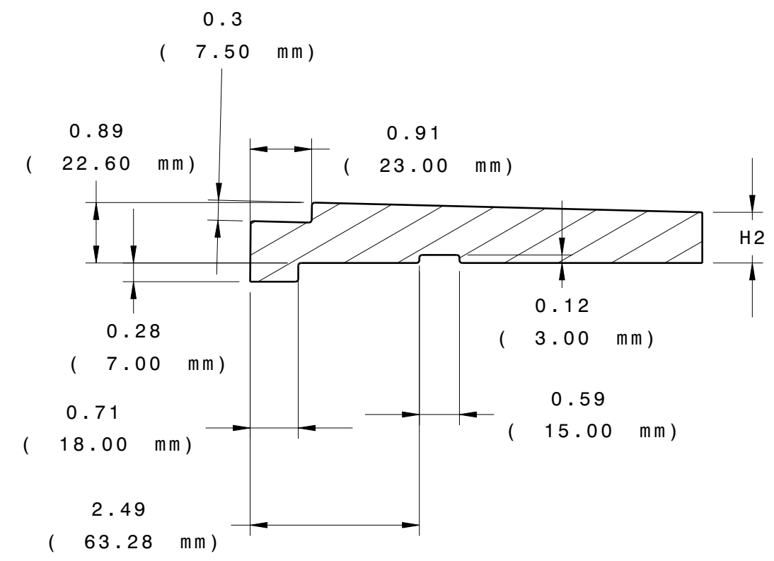
Section cut A-A
